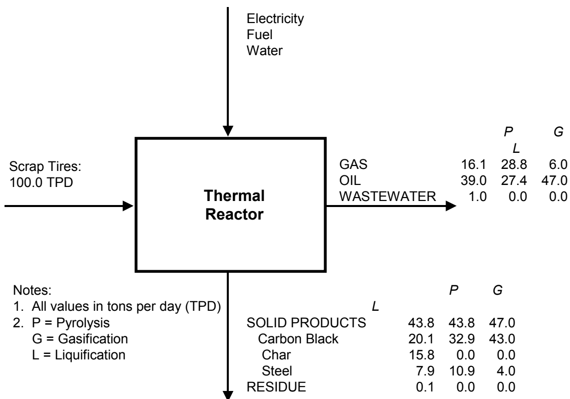
Figure 4-2. Typical Material Balance for Tire PGL Processes
