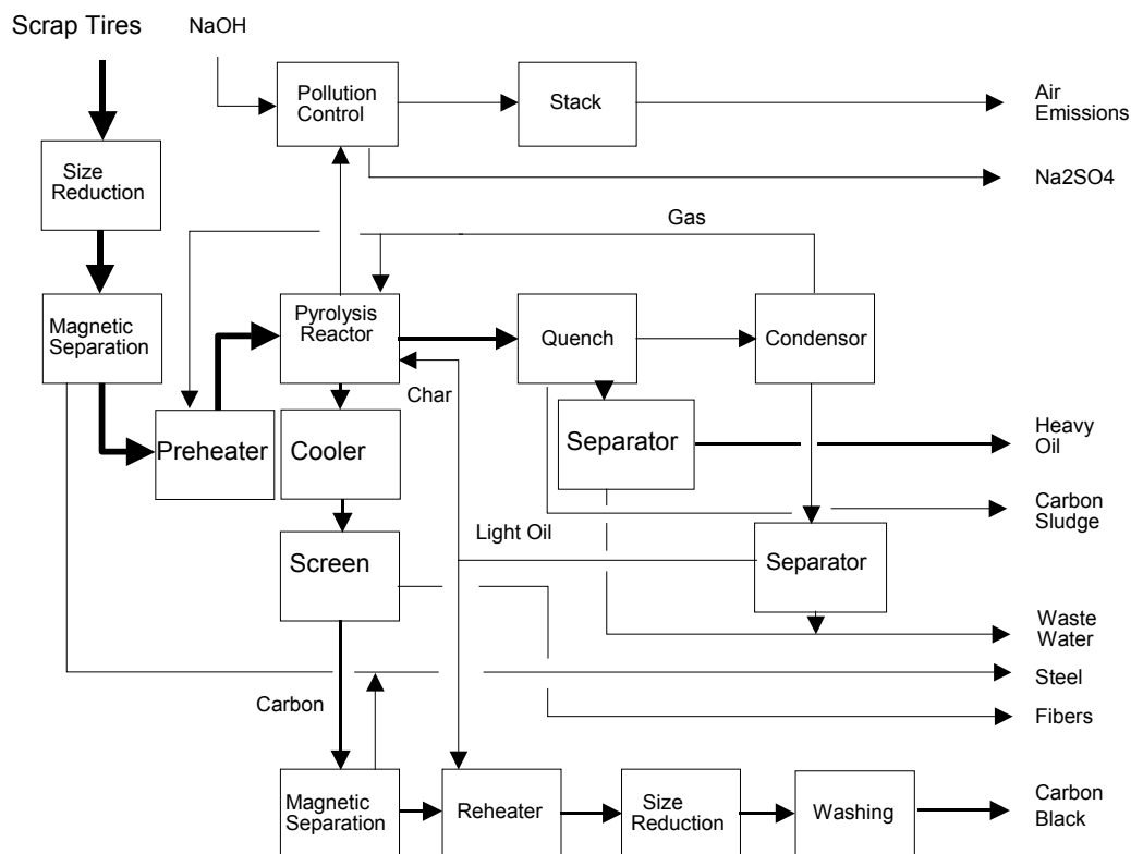
Figure 2-2. Flow Diagram - Typical Tire Pyrolysis System
